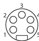
Connector B (J1-2)
